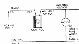
Figure 2 - Wiring
