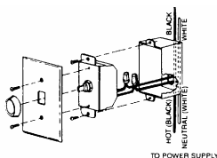
Figure 1 – Mounting
