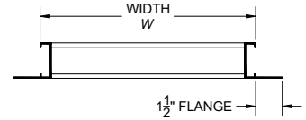
FRAME: FLANGE FRAME FLANGE-MOUNT (FM)
